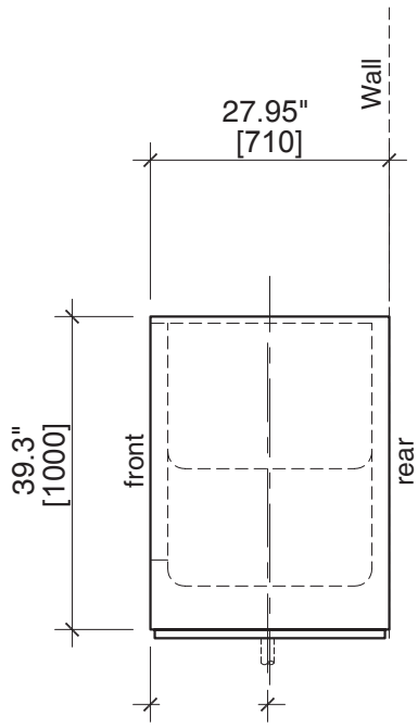
3 Side
